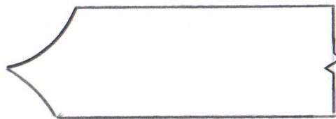
Over Ground Wing (Concave Grind On Wing)
